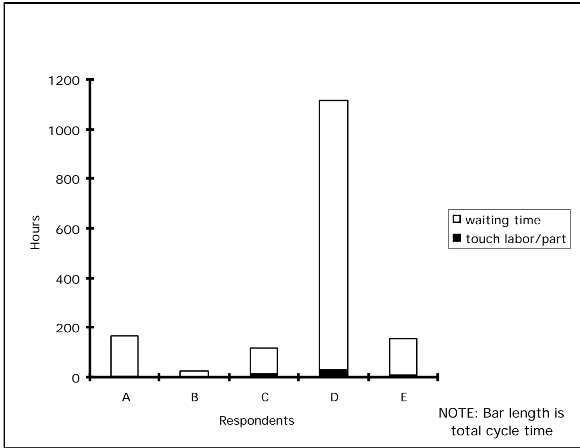
Figure 12: Electronic Sector - Cables/Harnesses
