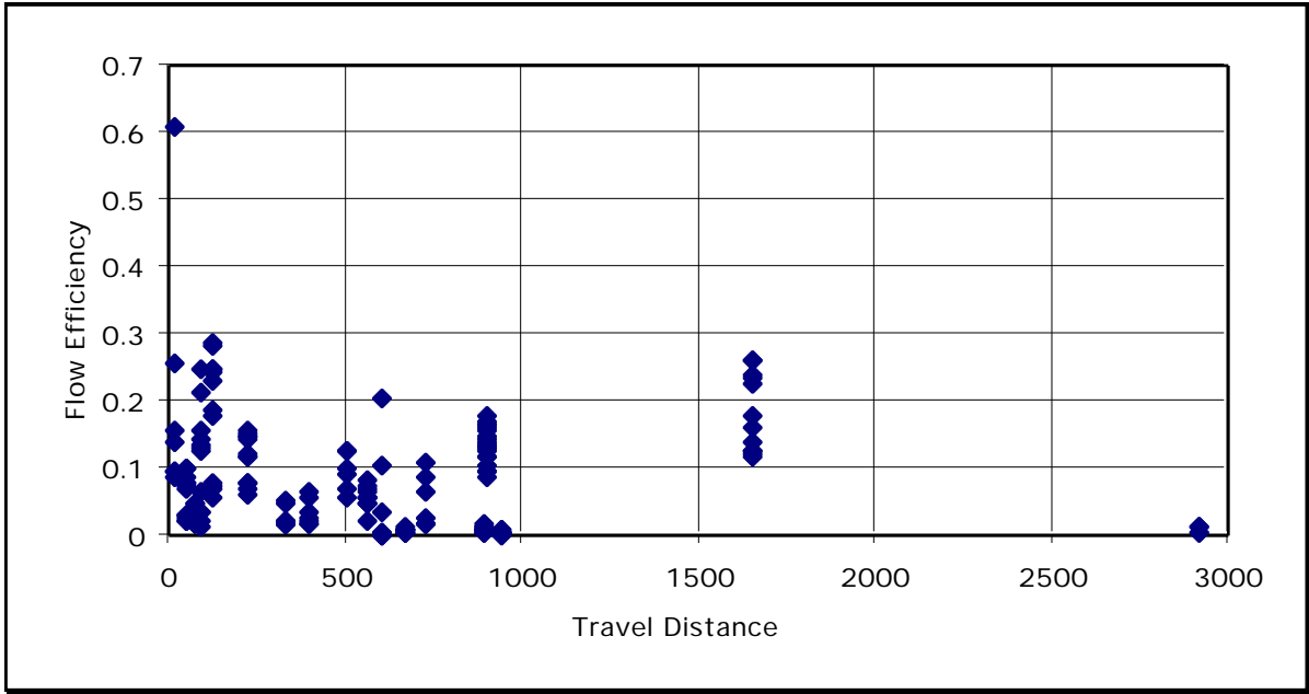
Figure 36: Flow Shop and Dedicated Line Flow Efficiencies versus Travel Distance
