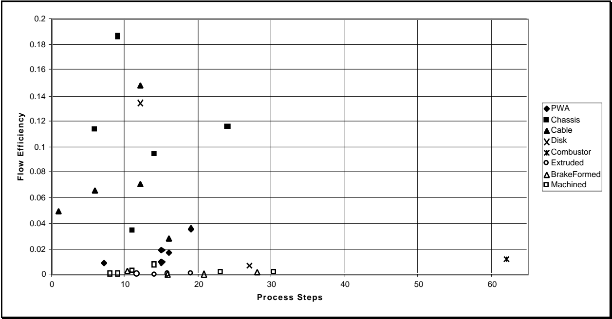
Figure 26: Flow Efficiency versus Process Steps
