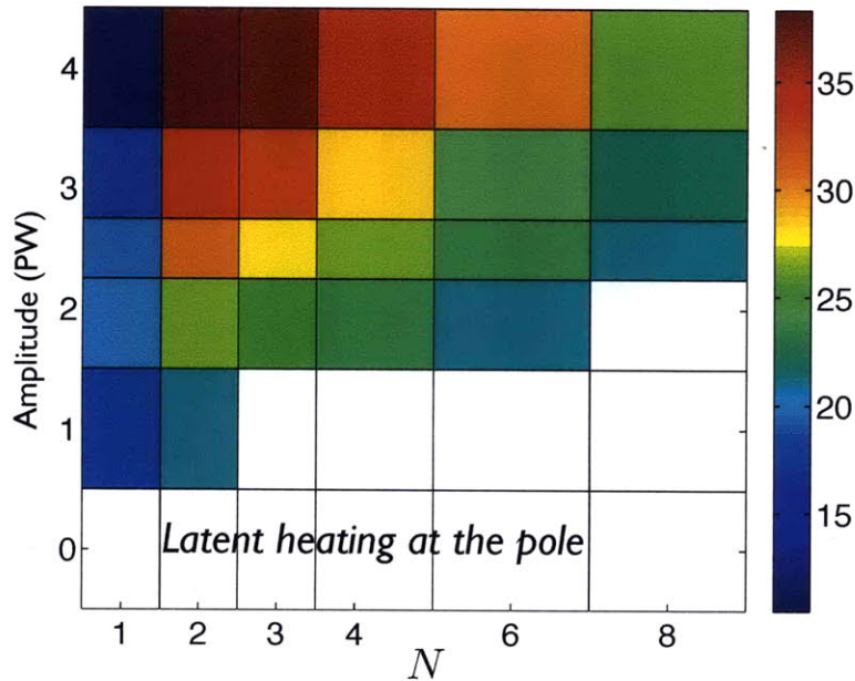
Figure 5-15: Latent heating at the pole in the slab ocean model as a function of OHT shape and magnitude. For all cases with an ice-free pole, convergence of latent heat is indicated by the colors in W m^{-2} . Nothing is plotted in the parts of the OHT parameter space for which an ice-free pole is not possible.
