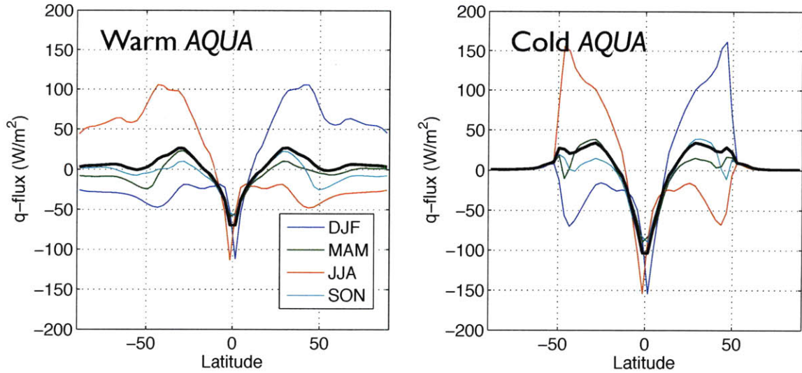
Figure 5-3: Seasonal and zonal mean q -fluxes diagnosed from the coupled Aqua . The thick black curves indicate annual means. These represent residuals of the heat budget for the first ocean model layer.
