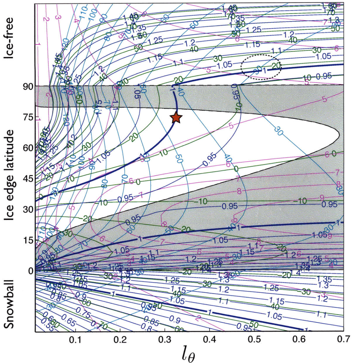
Figure 2-2: Solution space for the basic EB model as a function of the heat transport efficiency parameter l_\theta (horizontal axis) (with fixed radiative parameters). Blue contours represent q^* expressed as a fraction of the modern observed value (with the observed value emphasized). Multiple equilibria are represented by intersections between blue q^* contours and vertical lines; the unstable regions (where dq^*/dx_i < 0 ) are shaded. Green contours are global mean temperature ( ^\circ\text{C} ). Cyan contours are equator-to-pole temperature difference ( ^\circ\text{C} ). Magenta contours are poleward heat transport \mathcal{H} in units of PW. Vertical axis is the ice edge latitude. In the ice-free and ice-covered regions of the graph, the vertical spacing is chosen for graphical convenience and has no physical meaning. The red star indicates the approximate location of the observed climate in this phase space; the dashed circle indicates an approximate fit to the ice-free coupled Aquaplanet simulation discussed in Chapter 4.
