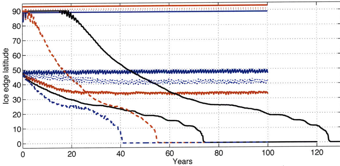
Figure 5-4: Evolution of the ice edge in slab ocean runs with prescribed ocean q -fluxes. Five runs are plotted starting from each of two initial conditions (Warm and Cold). The solid red (blue) curves indicate the full seasonal q -flux diagnosed from the coupled model Warm (Cold) state. Dotted lines indicate forcing by the annual mean of the full q -fluxes. Dashed lines indicate forcing by just the seasonal anomaly of the full q -fluxes. Black lines indicate zero q -flux, i.e. a swamp ocean. The “ice edge” here is actually global ice area, expressed as a latitude \tilde{\phi}_{ice} according to (4.1). The ice-free runs ( \tilde{\phi}_{ice} = 90^\circ ) are plotted with a slight offset for better visualization.
