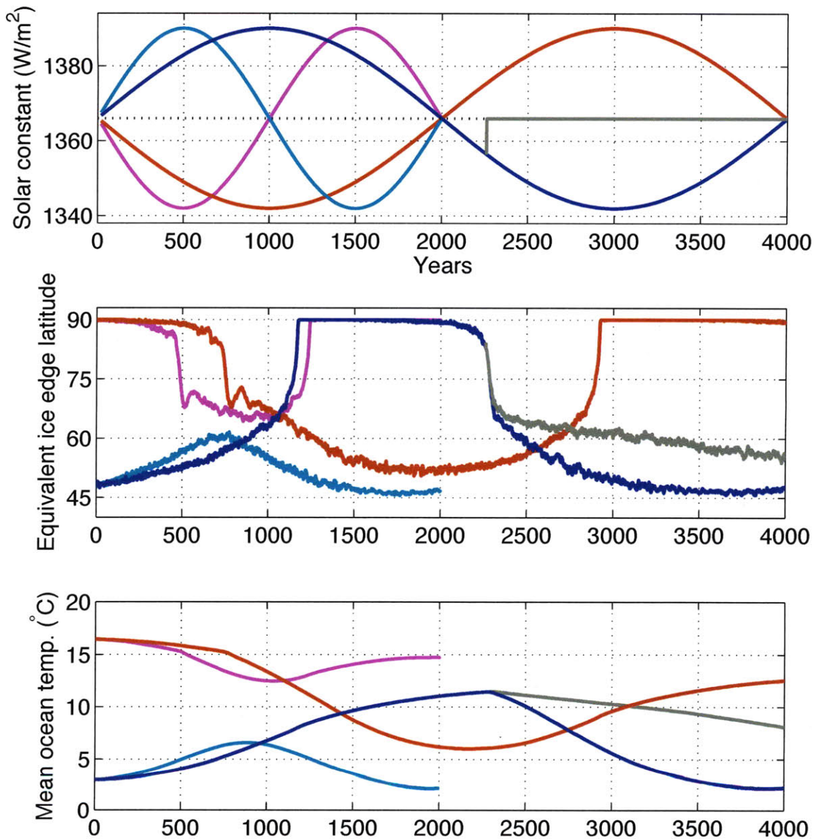
Figure 4-13: Transient climate change experiments in the coupled Aqua model. Upper panel shows the specified changes in solar constant (the external forcing). Middle panel shows equivalent ice edge latitude \tilde{\phi}_{ice} of the response (defined by (4.1)). Lower panel shows evolution of the global mean ocean temperature. The gray curve shows a model run in which solar constant is held at its reference value for the final 1740 years of the simulation.
