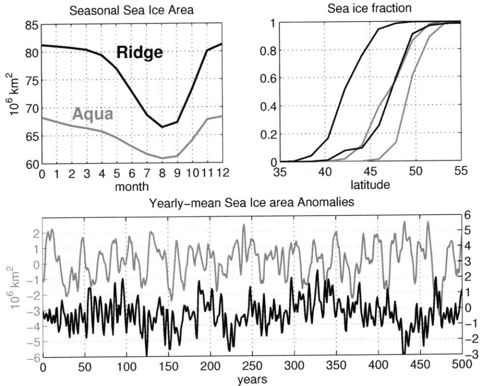
Figure 4-11: (top left) Seasonal cycle of the northern hemisphere sea ice extent (in millions km 2 ). (top right) Zonal mean northern hemisphere sea ice concentration in January and August. (bottom) Annual-mean sea ice extent anomaly in the Northern hemisphere as a function of time (note that, to remove some of the highest frequencies, the time-series are smoothed with a 1-2-1 running mean filter). Black and grey curves correspond to Ridge and Aqua , respectively. Reproduced from Ferreira et al. (2010b).
