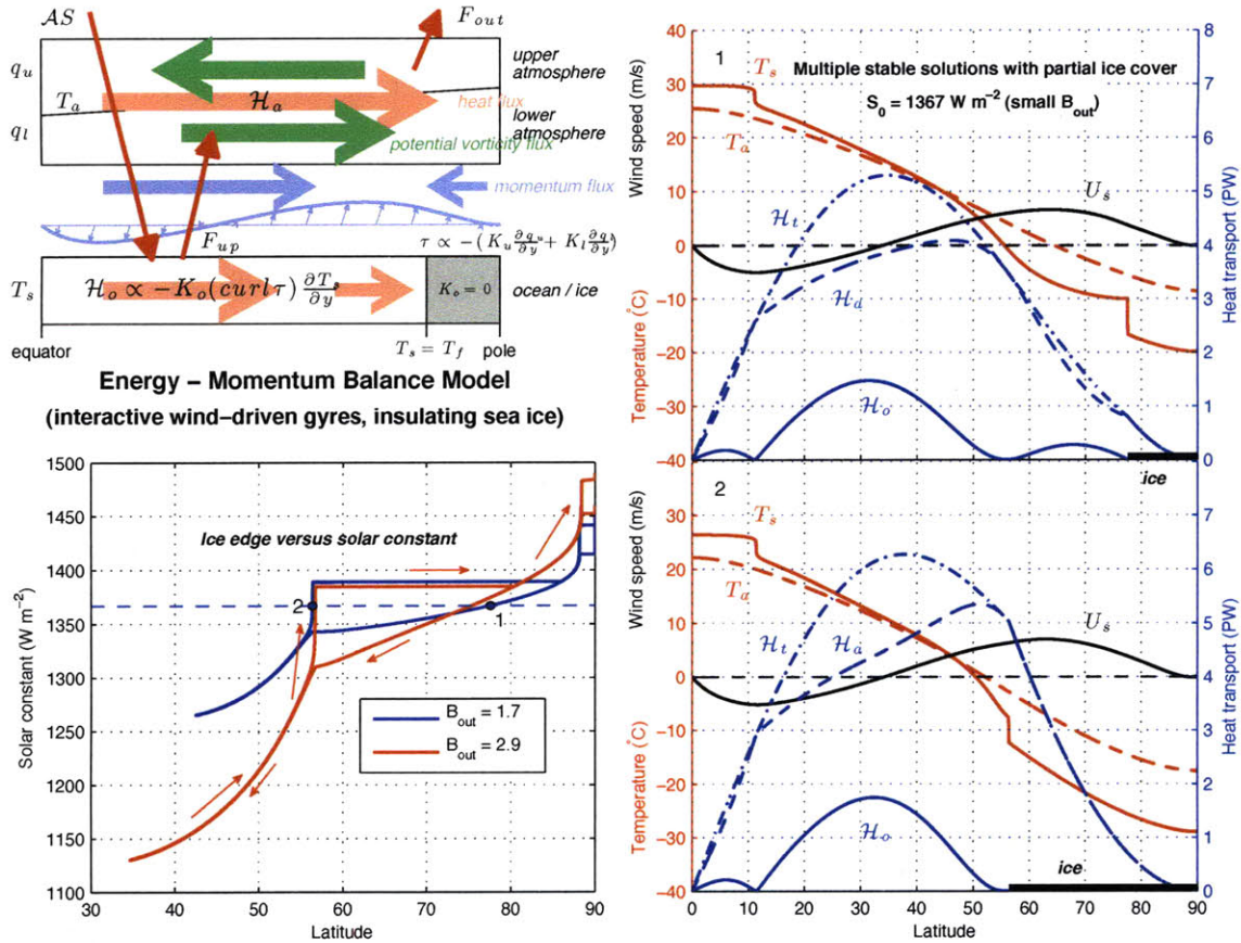
Figure 3-1: Solutions from the Energy-Momentum Balance Model. The atmosphere is now represented by two layers of QGPV (equations (3.9)), with the temperature T_a in thermal wind balance with the vertical wind shear. Meridional fluxes of heat and angular momentum (sketched in red and blue respectively) are implicitly represented by a meridional eddy QGPV flux (sketched in green). The ocean is driven by \tau , generated interactively by the atmospheric model (the westerlies being maintained by the convergence of momentum fluxes in mid-latitudes); otherwise the ocean is identical to that shown in Fig. 2-4. The model supports multiple stable ice edges, as illustrated in the top right and bottom right. The S_0 - \phi_i relationships (lower left) are similar to those in the AO-EBM with fixed wind-driven gyres (Fig. 2-4). A grayscale version of this figure appears in Rose and Marshall (2009).
