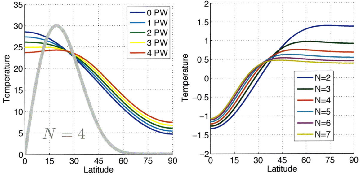
Figure 5-8: The effects of OHT on atmospheric temperature in the AO-EBM. Left panel: \theta vs. latitude for different amplitudes of OHT, with fixed spatial structure ( N = 4 ). Right panel: the component of \theta due to OHT forcing, as function of the meridional scale parameter N . Plotted in units of ^{\circ}\text{C} per PW of OHT.
