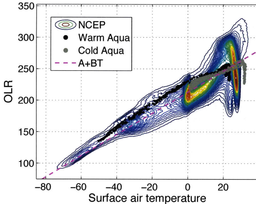
Figure C-3: Scatterplots of OLR versus surface air temperature in the NCEP reanalysis and in two Aquaplanet model climatologies. The reanalysis data are binned and plotted as a 2D density histogram – warmer colored contours indicate higher densities of data points. Black and gray dots are from the zonally averaged climatologies of the Warm and Cold Aquaplanet simulations. The dashed line is the best fit to the reanalysis data with A = 213 \text{ W m}^{-2} , B = 1.68 \text{ W m}^{-2} \text{ }^{\circ}\text{C}^{-1} .
