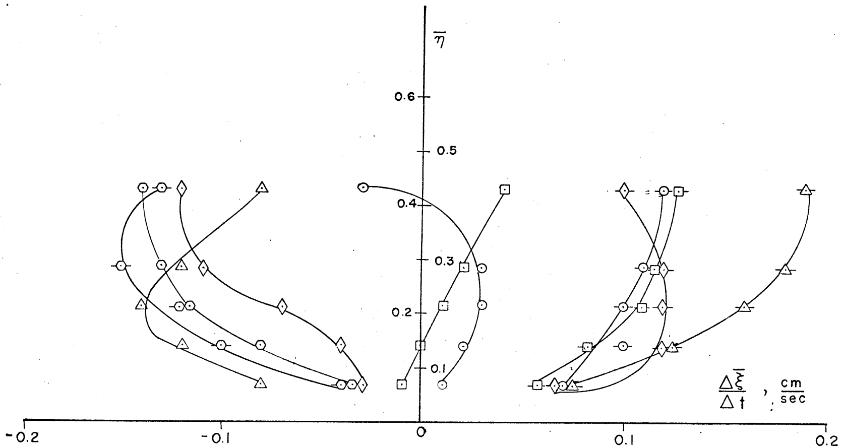
Fig. 58. Vertical distribution of velocity near the bottom at station 5. a_o = 0.2 cm, \omega = 0.105 cps, N = 0.155 cps, \theta = 30 deg, x_c = 100.0 cm.
