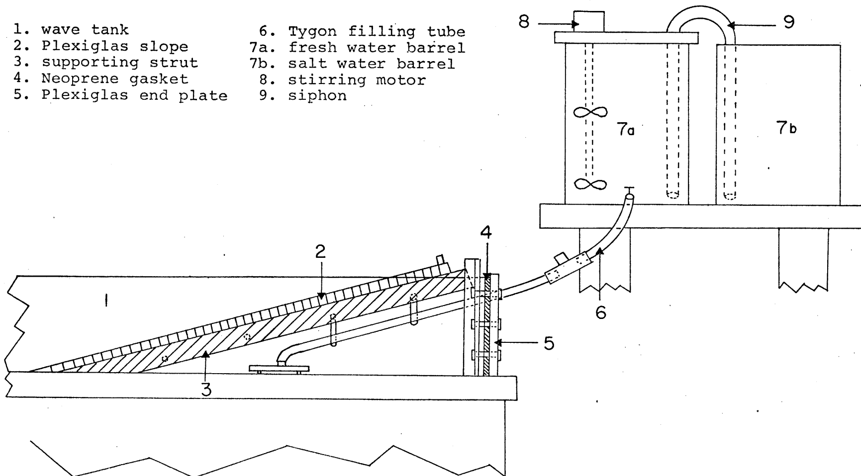
Fig. 1. Wave tank and filling system.
