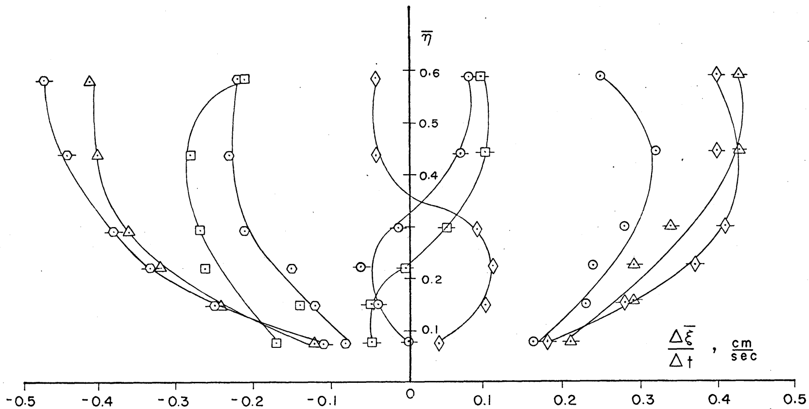
Fig. 55. Vertical distribution of velocity near the bottom at station 2. a_0 = 0.2 cm, \omega = 0.105 cps, N = 0.155 cps, \alpha = 30 deg, x_c = 23.0 cm.
