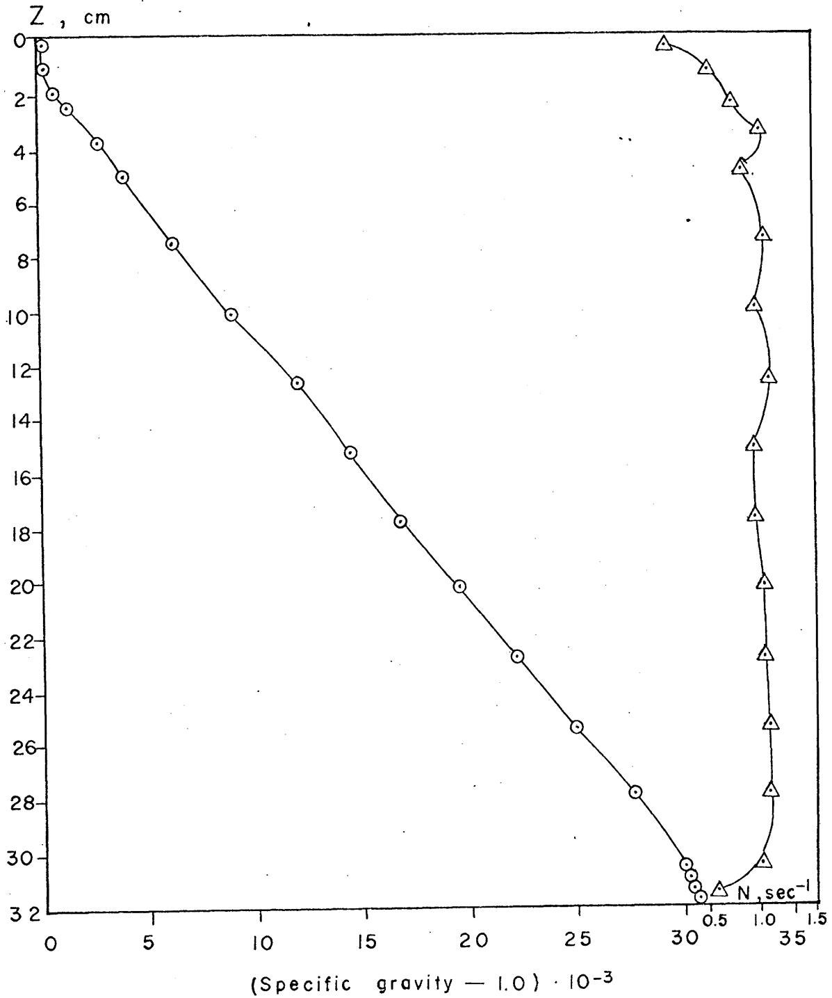
Fig. 9. Typical specific gravity variation with depth. Data from exp. group 2; computed vertical distribution of Brunt Vaisala frequency is also shown.
