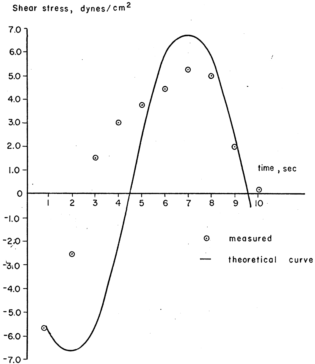
Fig. 61 a. Experimental and theoretical values of bed shear stress \tau_0 at station 1. The experimental values were obtained for each second of time t during one wave cycle.
