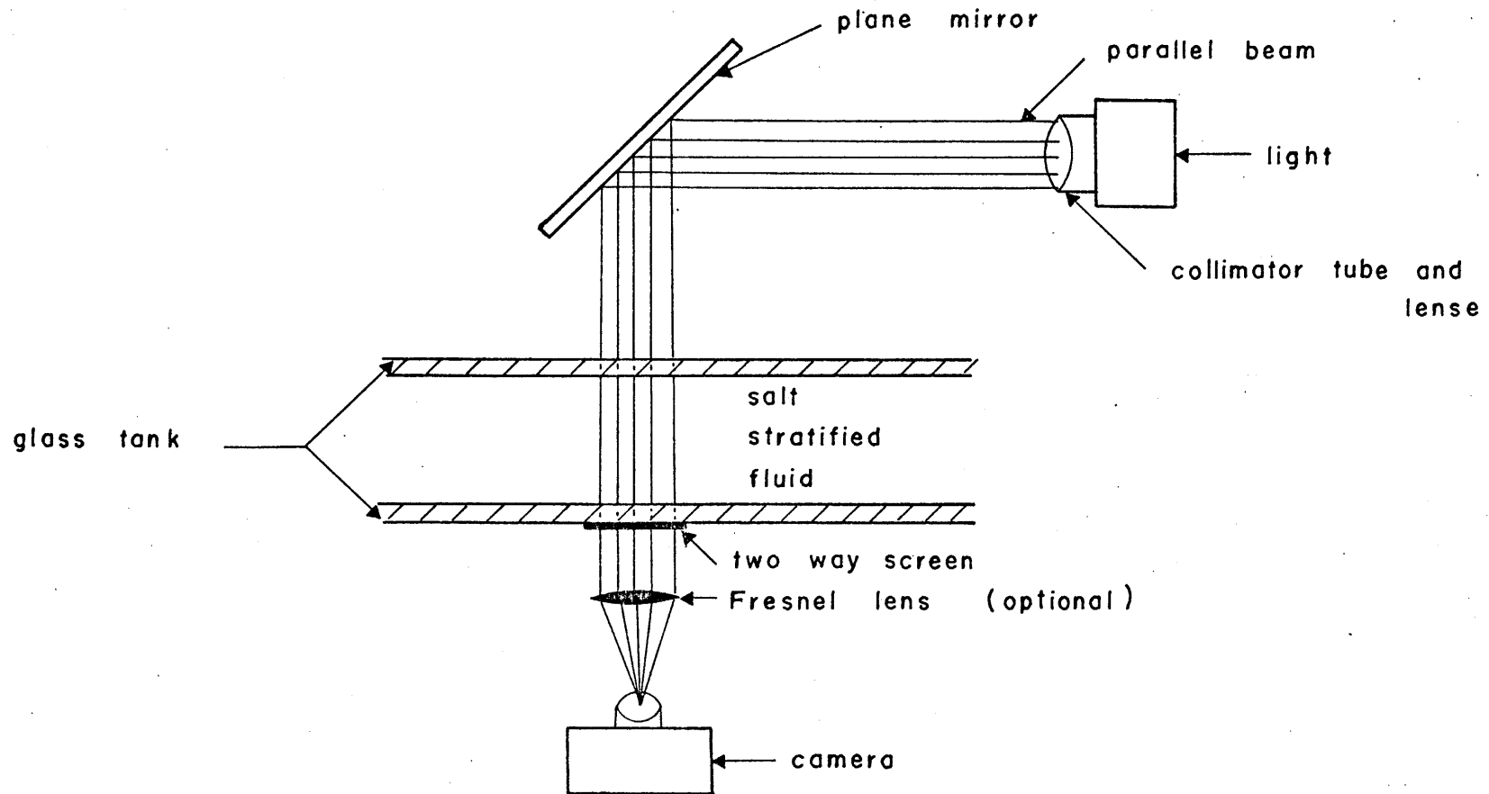
Fig. 6. Schematic of shadowgraph system.
