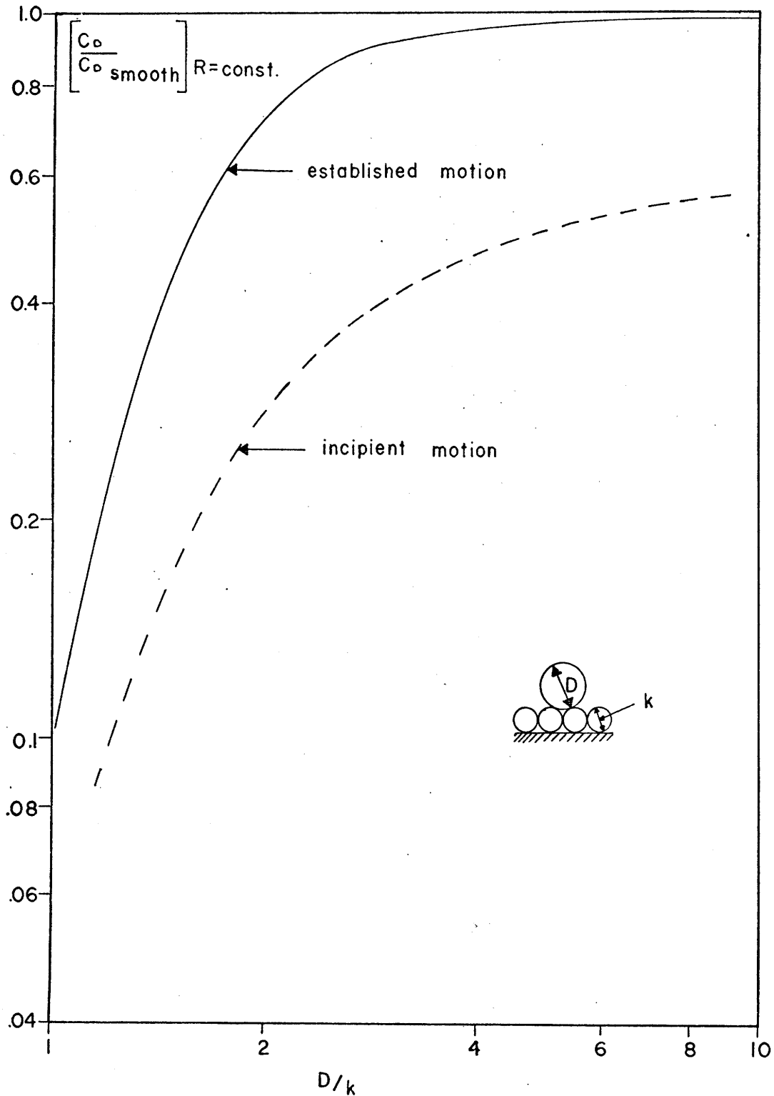
FIG. 82. Effect of bed-particle geometry on the resistance coefficients for spheres (after Eagleson and Dean, 1959).
