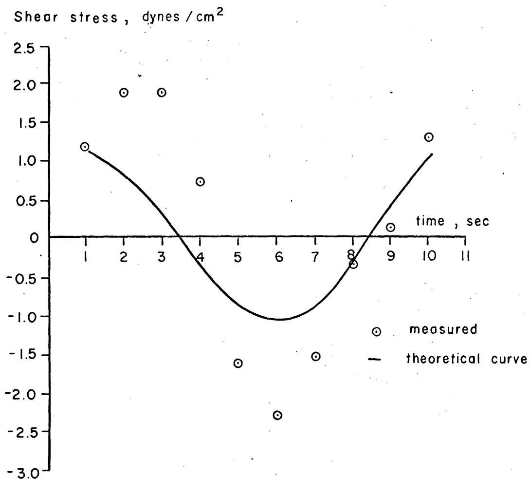
Fig. 61 c. Experimental and theoretical values of bed shear stress \tau_0 at station 3. The experimental values were obtained for each second of time t during one wave cycle.
