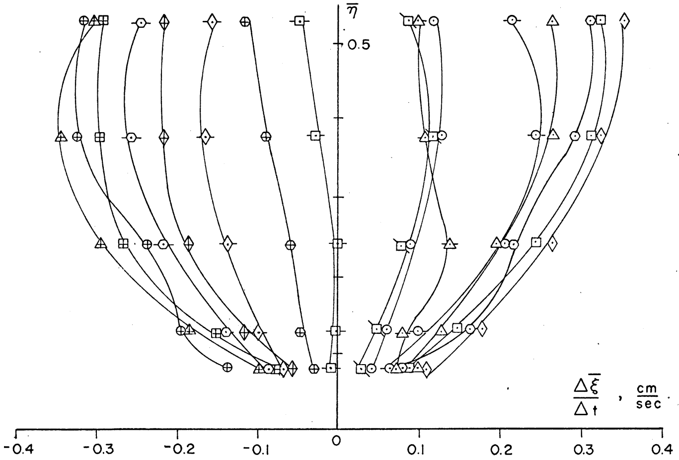
FIG 73b. Velocity - depth profiles at station 4, \gamma > c .
