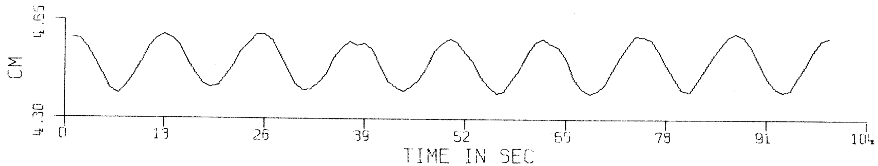
Fig. 10. Raw data plotted for wave maker and conductivity probe output. Mean not removed. (Data from Exp. Group 5)
