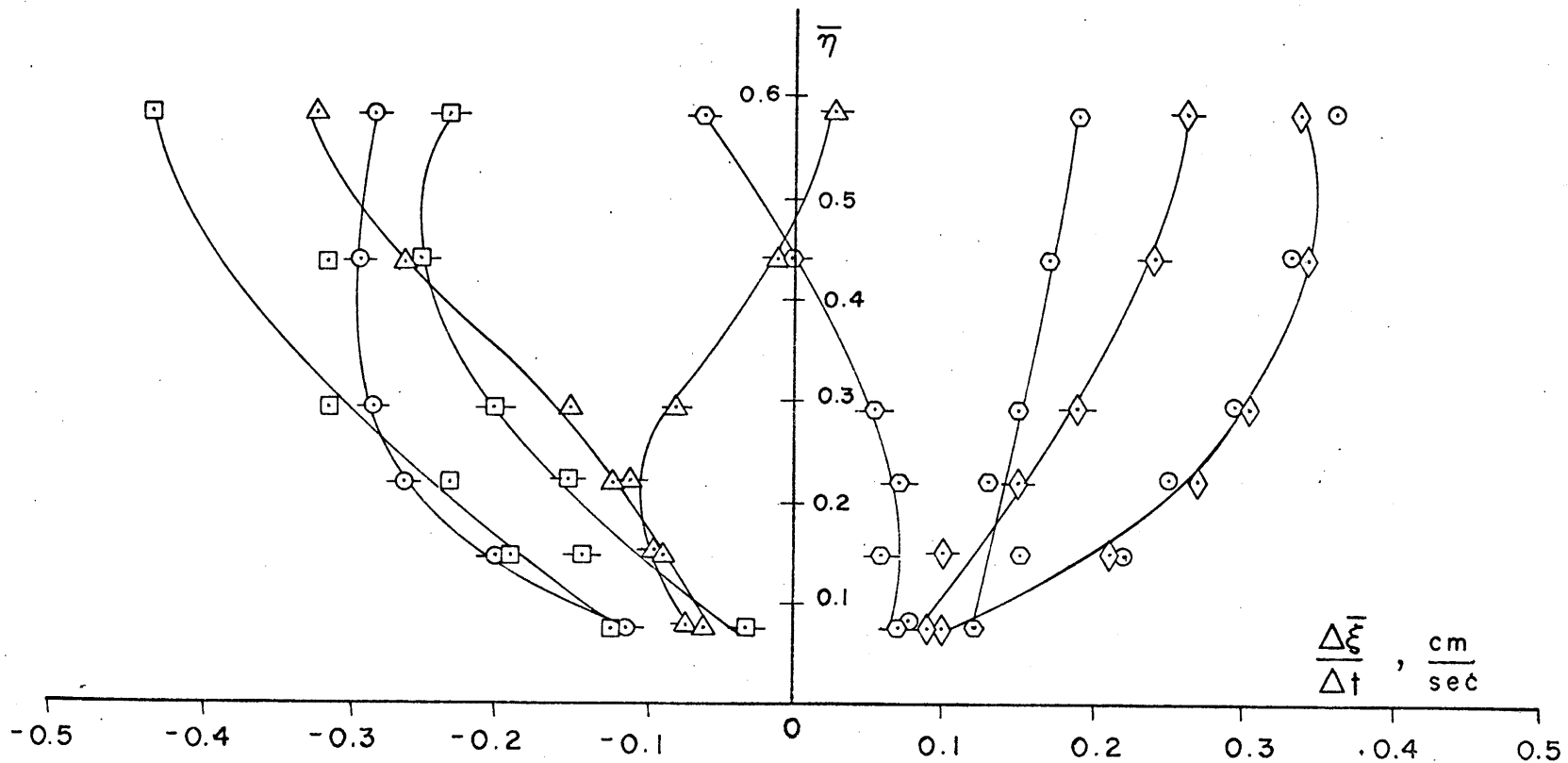
Fig. 56. Vertical distribution of velocity near the bottom at station 3. a_0 = 0.2 cm, \omega = 0.105 cps, N = 0.155 cps, \alpha = 30 deg, x_c = 36.0 cm.
