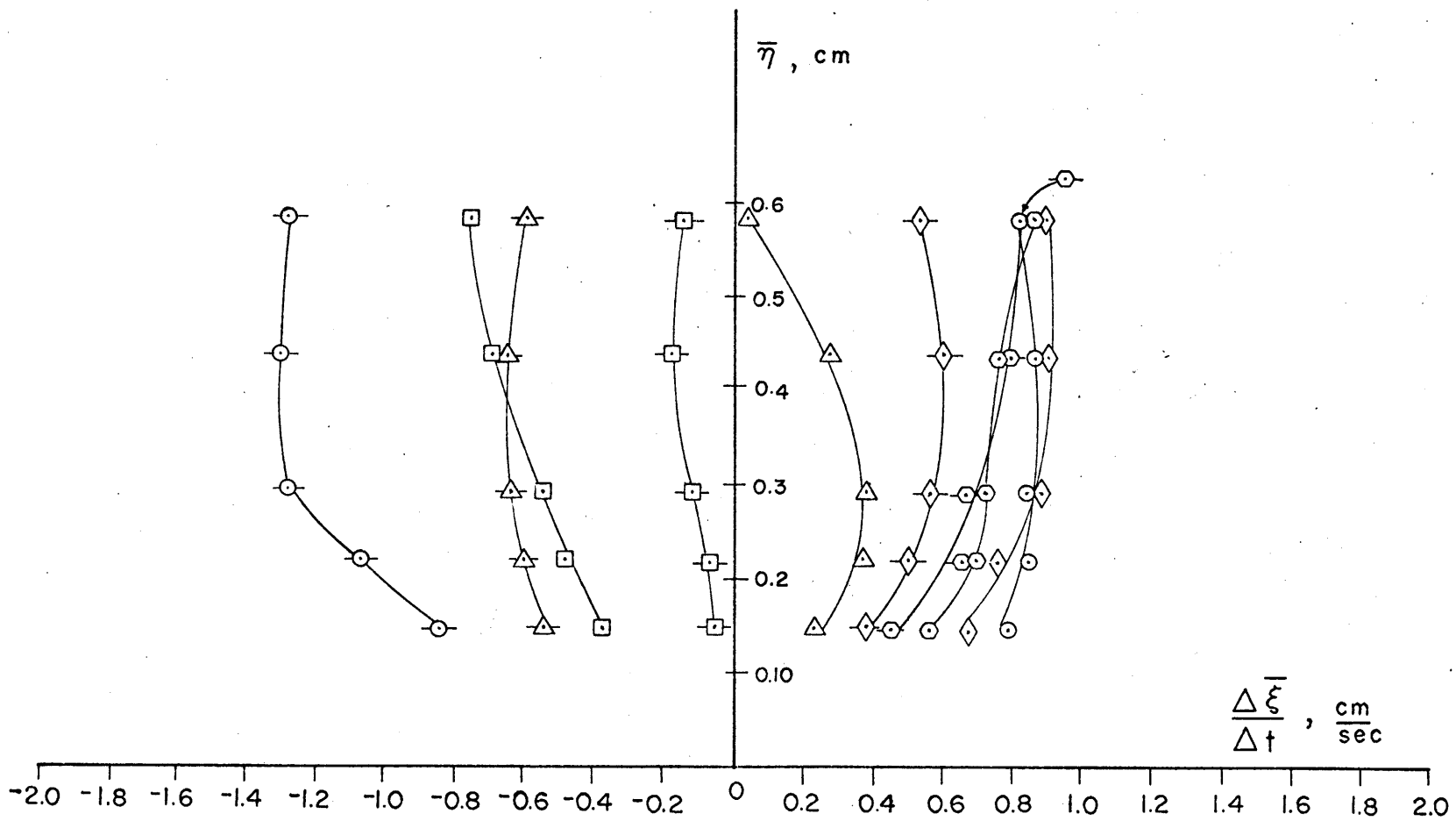
Fig. 54. Vertical distribution of velocity near the bottom at station 1. a_0 = 0.2 cm, \omega = 0.105 cps, N = 0.155 cps, \alpha = 30 deg, x_c = 8.7 cm.
