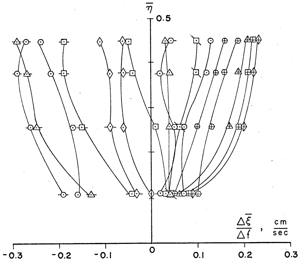
FIG. 73a. Velocity - depth profiles at station 1, \gamma > c .
