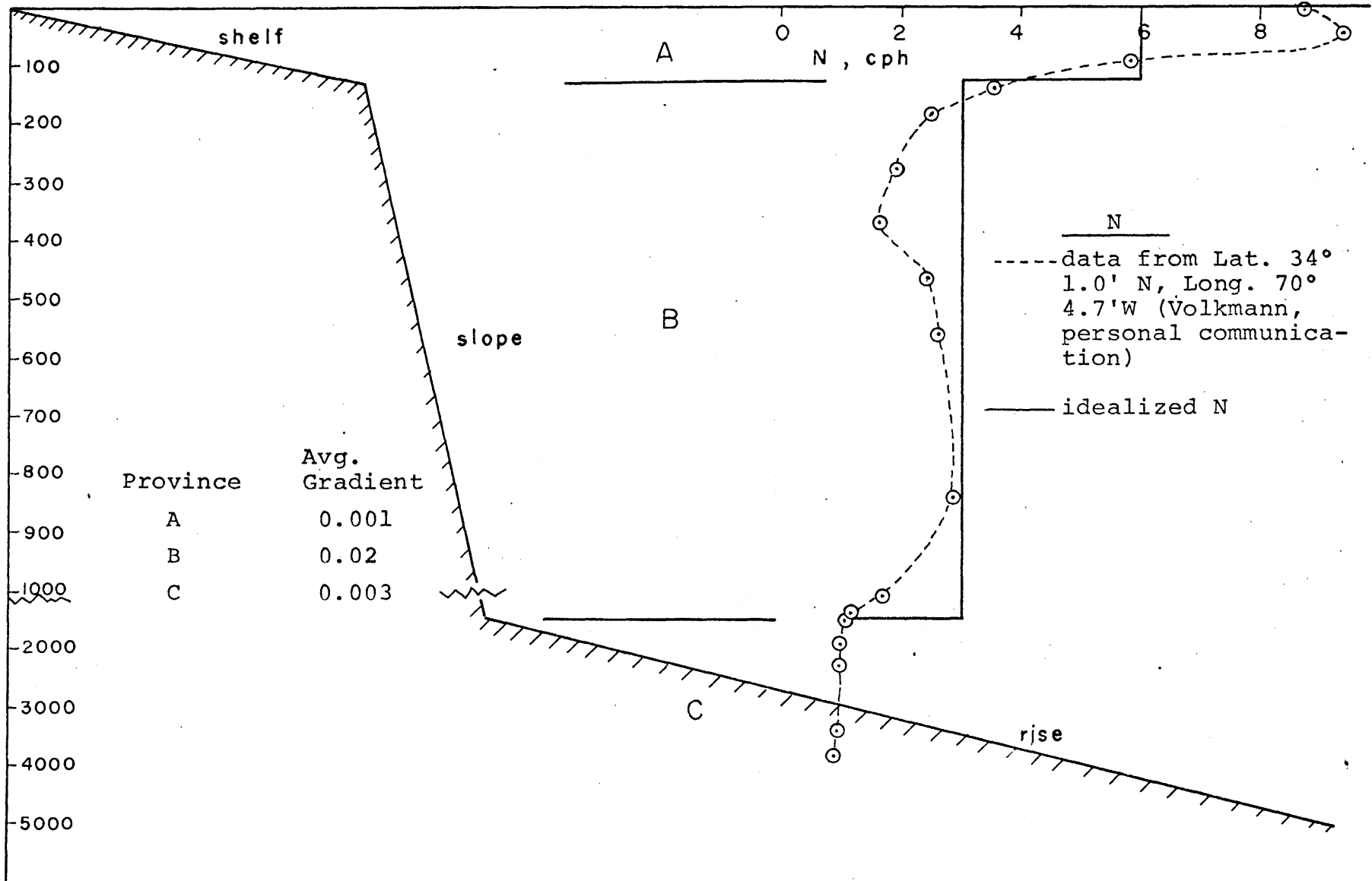
FIG. 78. Idealized cross section of continental margin. Actual and idealized distribution of Brunt-Vaisala frequency are also shown.
