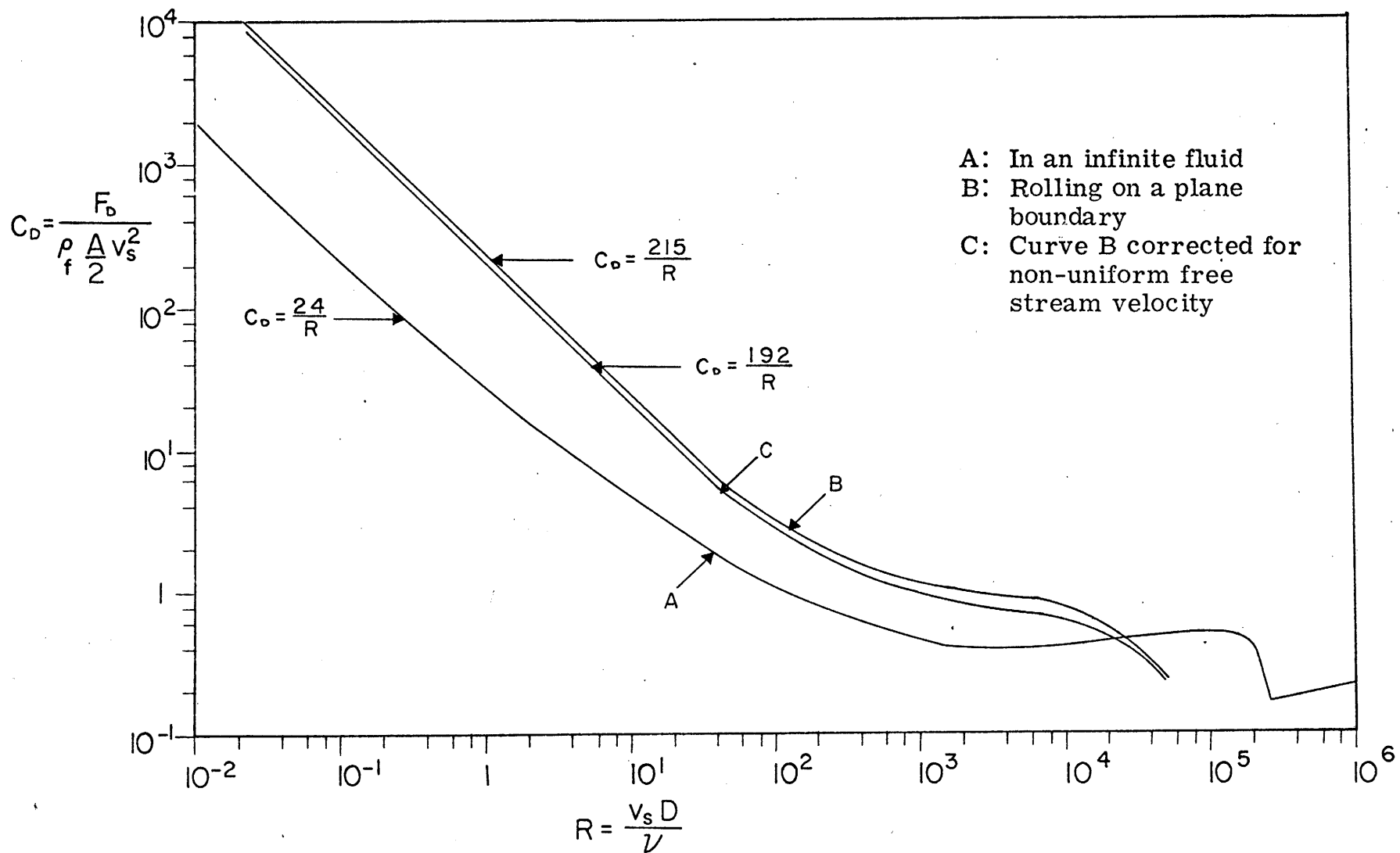
FIG. 81. Resistance coefficients C_D for spheres (after Eagleson and Dean, 1959).
