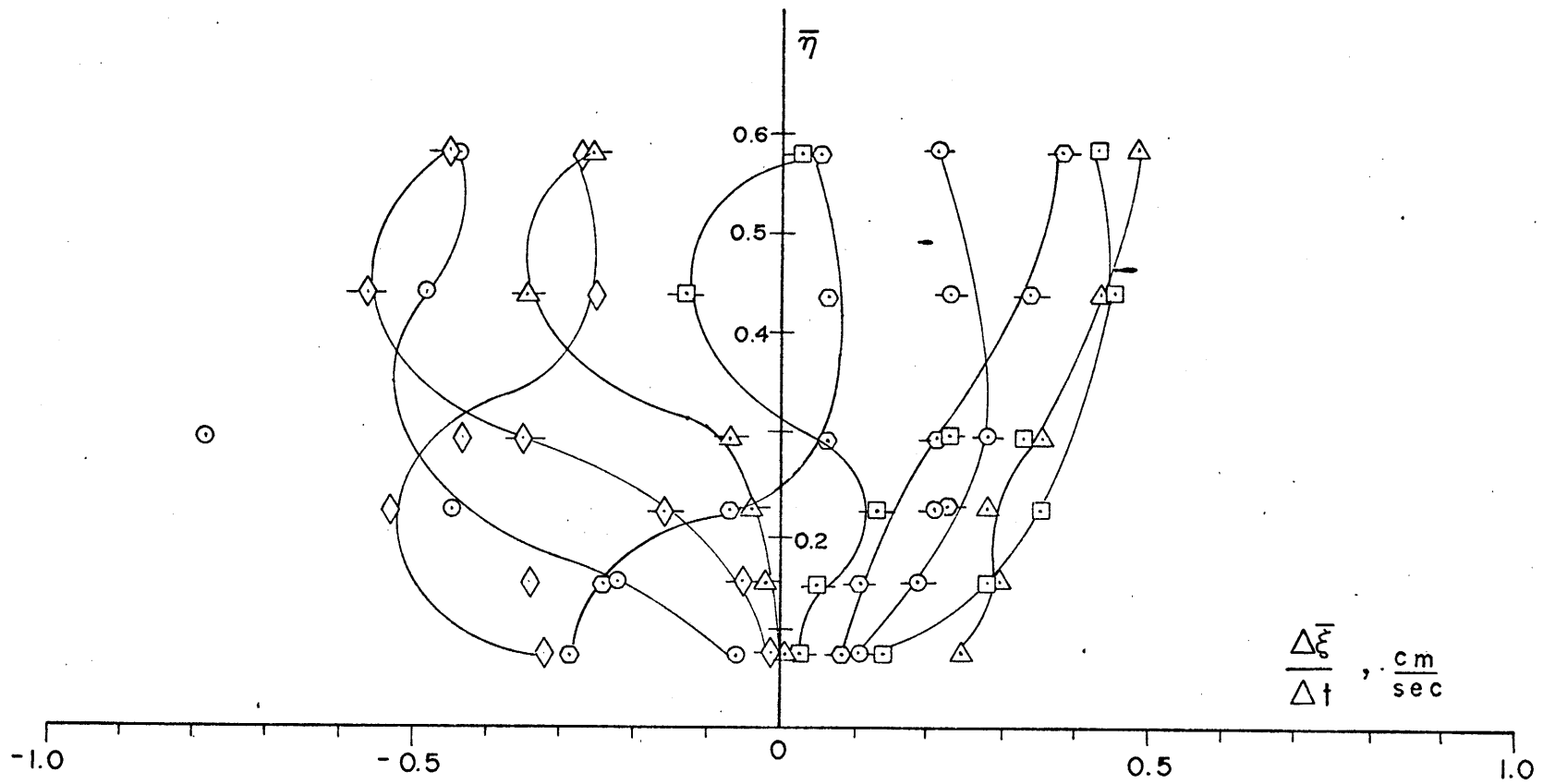
Fig. 57. Vertical distribution of velocity near the bottom at station 4. a_0 = 0.2 cm, \omega = 0.105 cps, N = 0.155 cps, \alpha = 30 deg, x_c = 51.0 cm.
