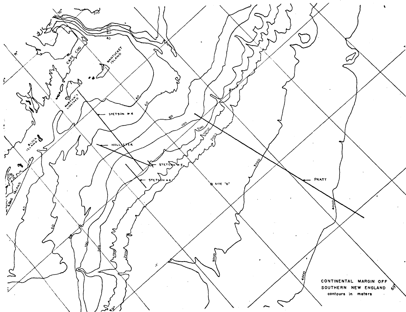
Fig. 76. Bathymetry off southern New England.
