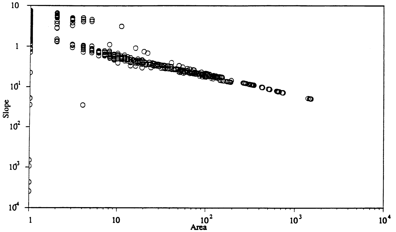
Figure 3-46: Area-Slope Renormalization. All Nodes Included. Case 33 Before Dynamic Equilibrium. Time 6000
