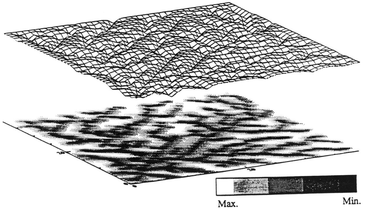
Figure 3-56: Elevations at Time 7000. Case BR661SATU10
