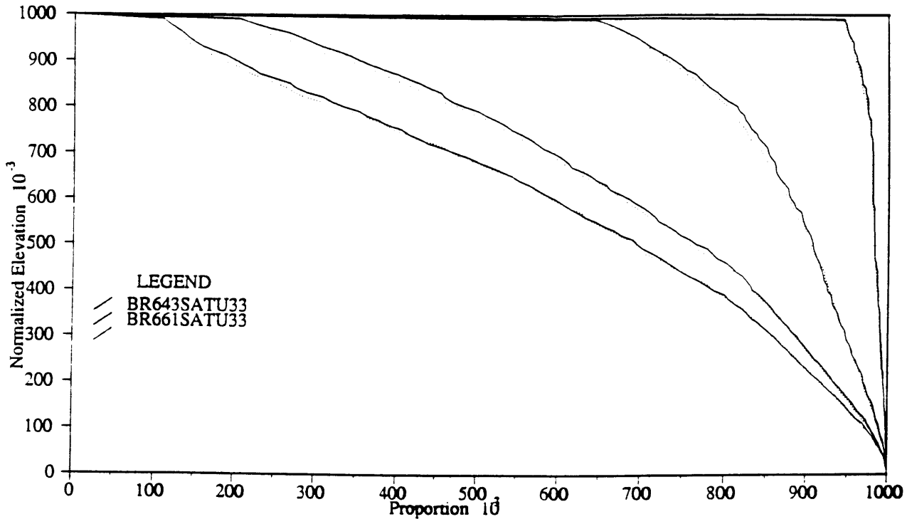
Figure 3-60: Hypsometric Curve Evolution. Cases BR643SATU33 and BR661SATU33
