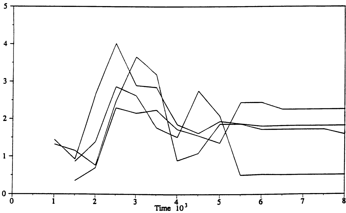
Figure 3-27: Strahler Length Ratio. Order 2-3
