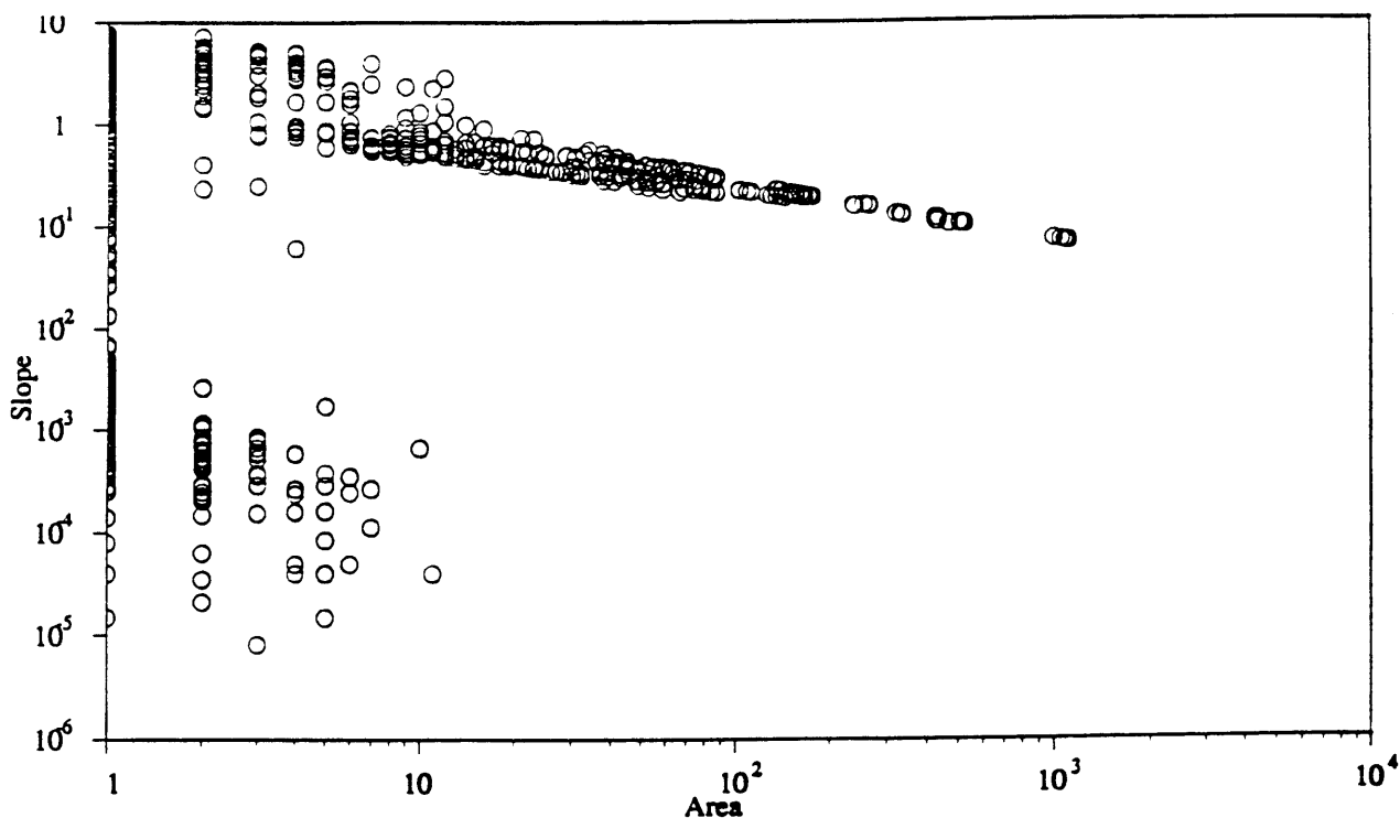
Figure 3-45: Area-Slope Renormalization. All Nodes Included. Case 33 Before Dynamic Equilibrium. Time 4000
