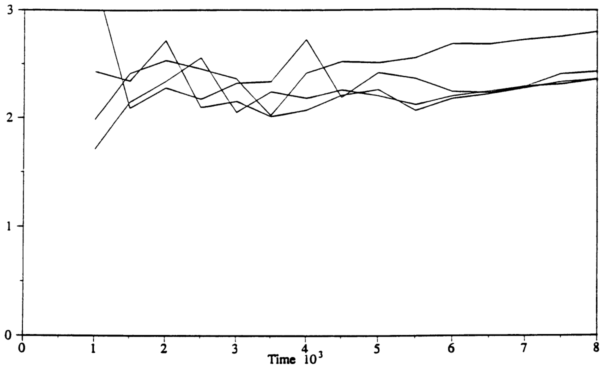
Figure 3-28: Strahler Slope Ratio. Order 1-2
