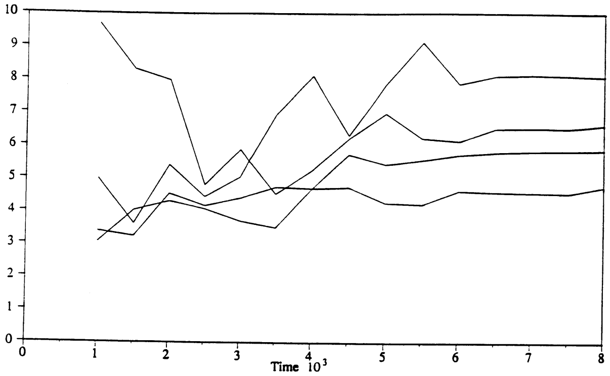
Figure 3-30: Strahler Area Ratio. Order 1-2
