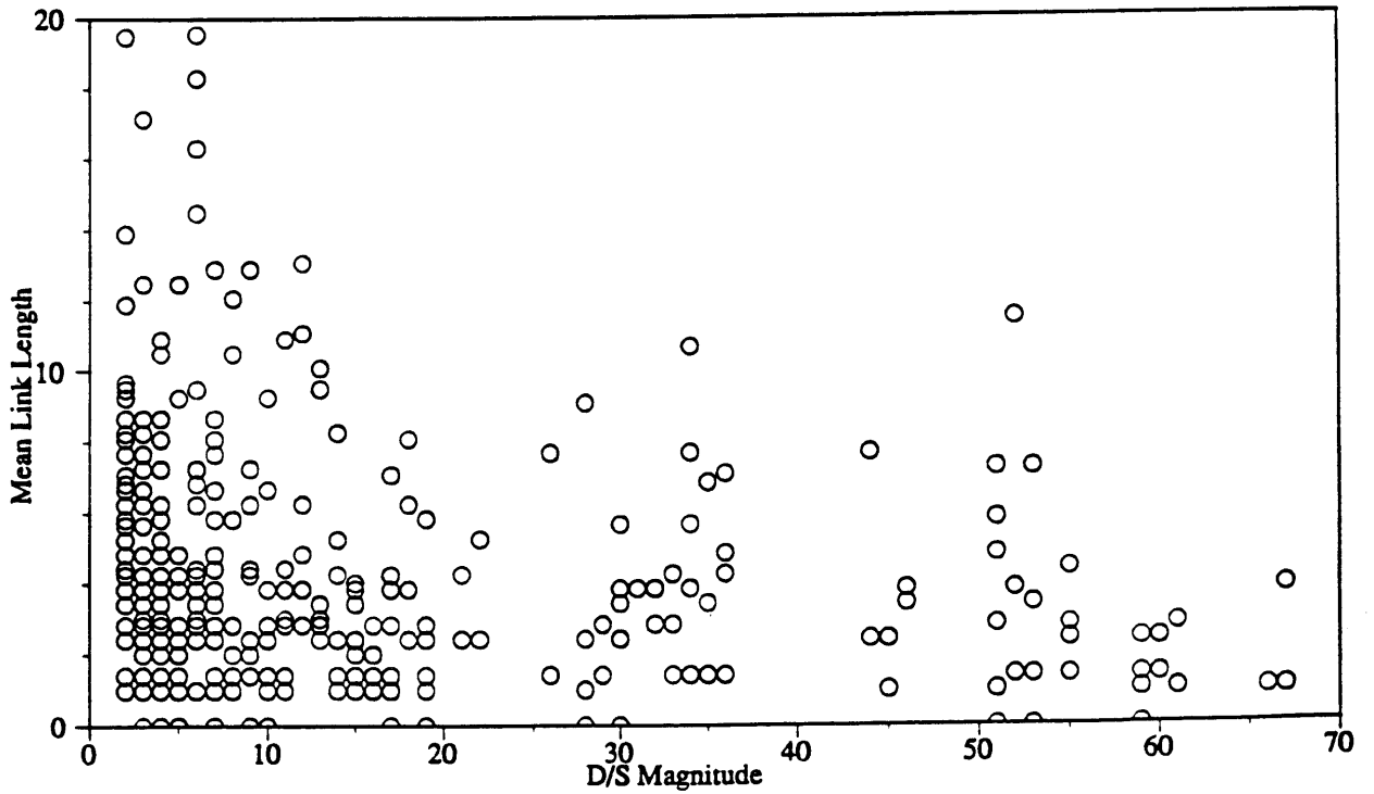
Figure 3-50: Link Length vs. Magnitude. Cases 10,34,35,36
