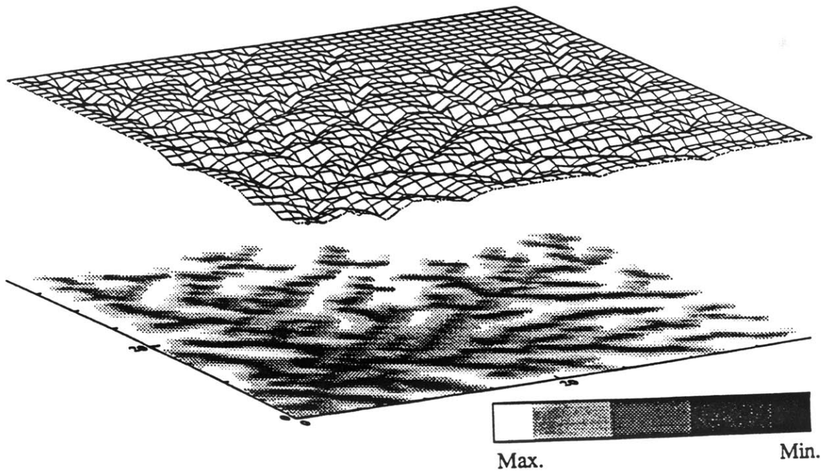
Figure 3-55: Elevations at Time 5000. Case BR661SATU10
