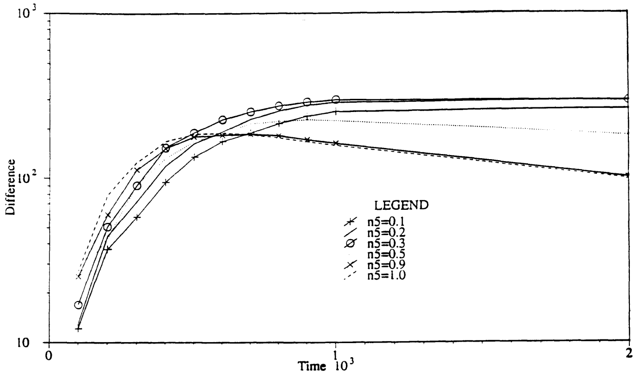
Figure 4-31: Relief Difference Under n 5 Variations During Network Growth
