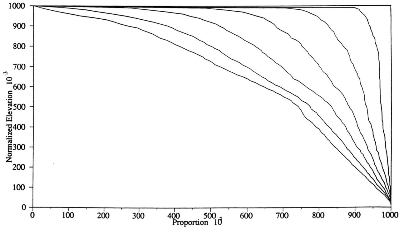
Figure 3-66: Hypsometric Curve Evolution TSC=0.276 \times 10^3
