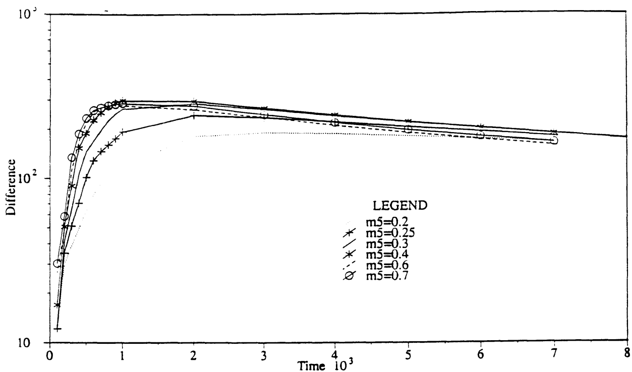
Figure 4-27: Relief Difference Under m 5 Variations
