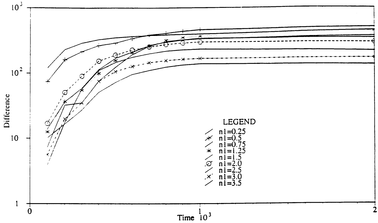
Figure 4-19: Relief Difference Under n_1 Variations During Network Growth
