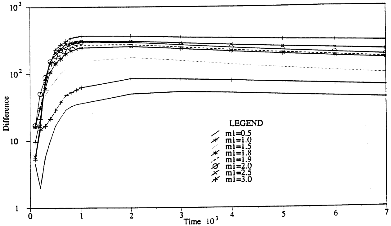
Figure 4-12: Relief Difference Under m_1 Variations
