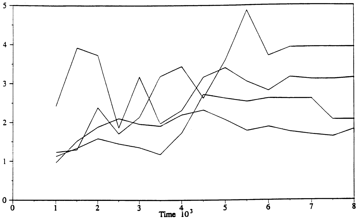
Figure 3-26: Strahler Length Ratio. Order 1-2
