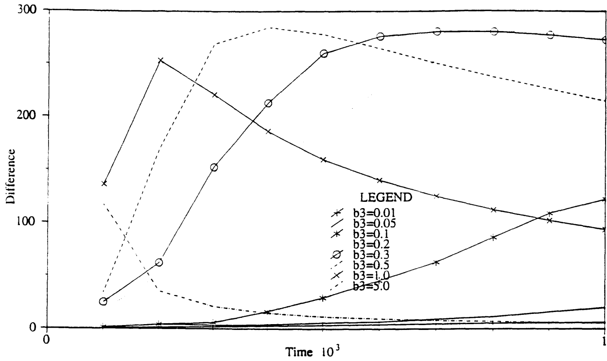
Figure 4-23: Relief Difference Under \beta_3 Variations. Arithmetic Scale
