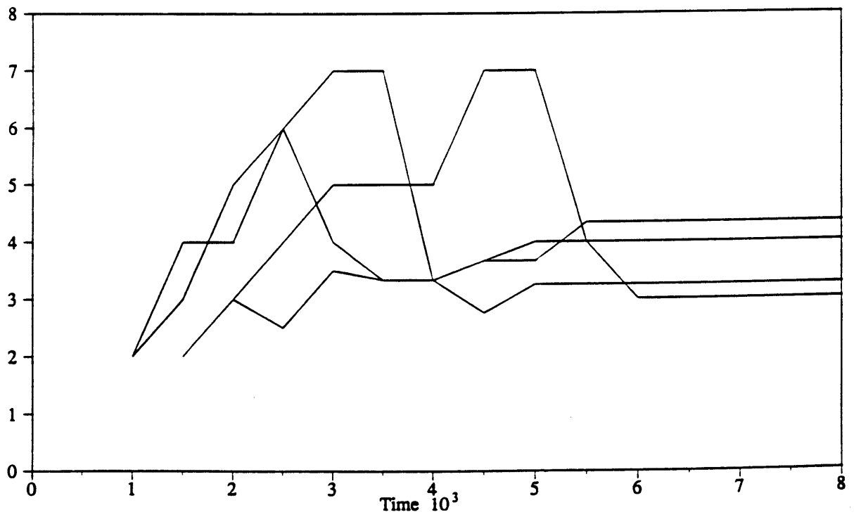
Figure 3-25: Strahler Bifurcation Ratio. Order 2-3
