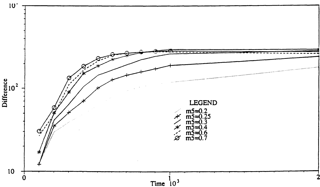
Figure 4-28: Relief Difference Under m 5 Variations During Network Growth
