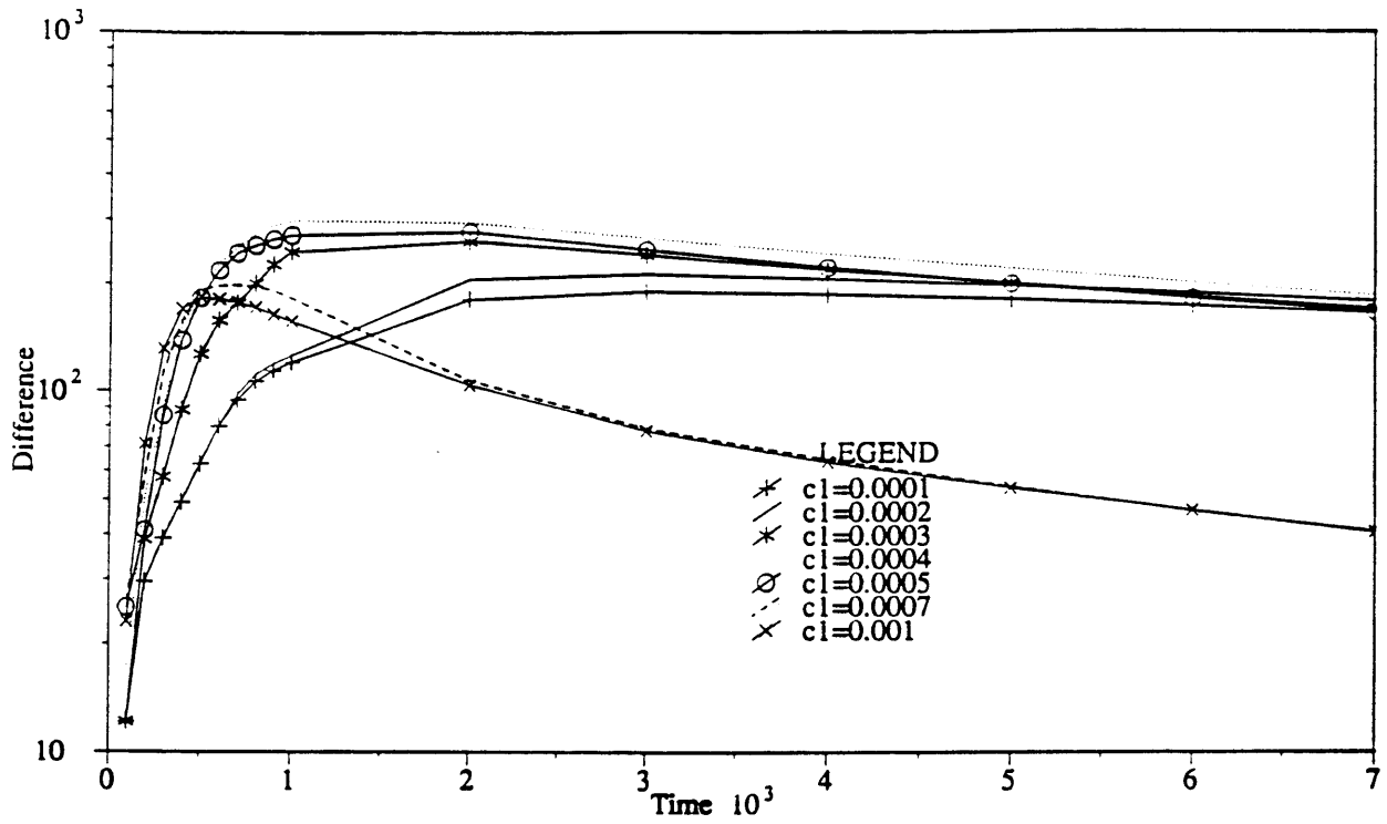
Figure 4-15: Relief Difference Under c 1 Variations
