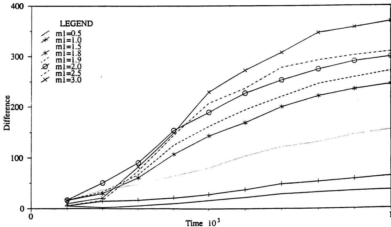
Figure 4-14: Relief Difference Under m 1 Variations. Arithmetic Scale
