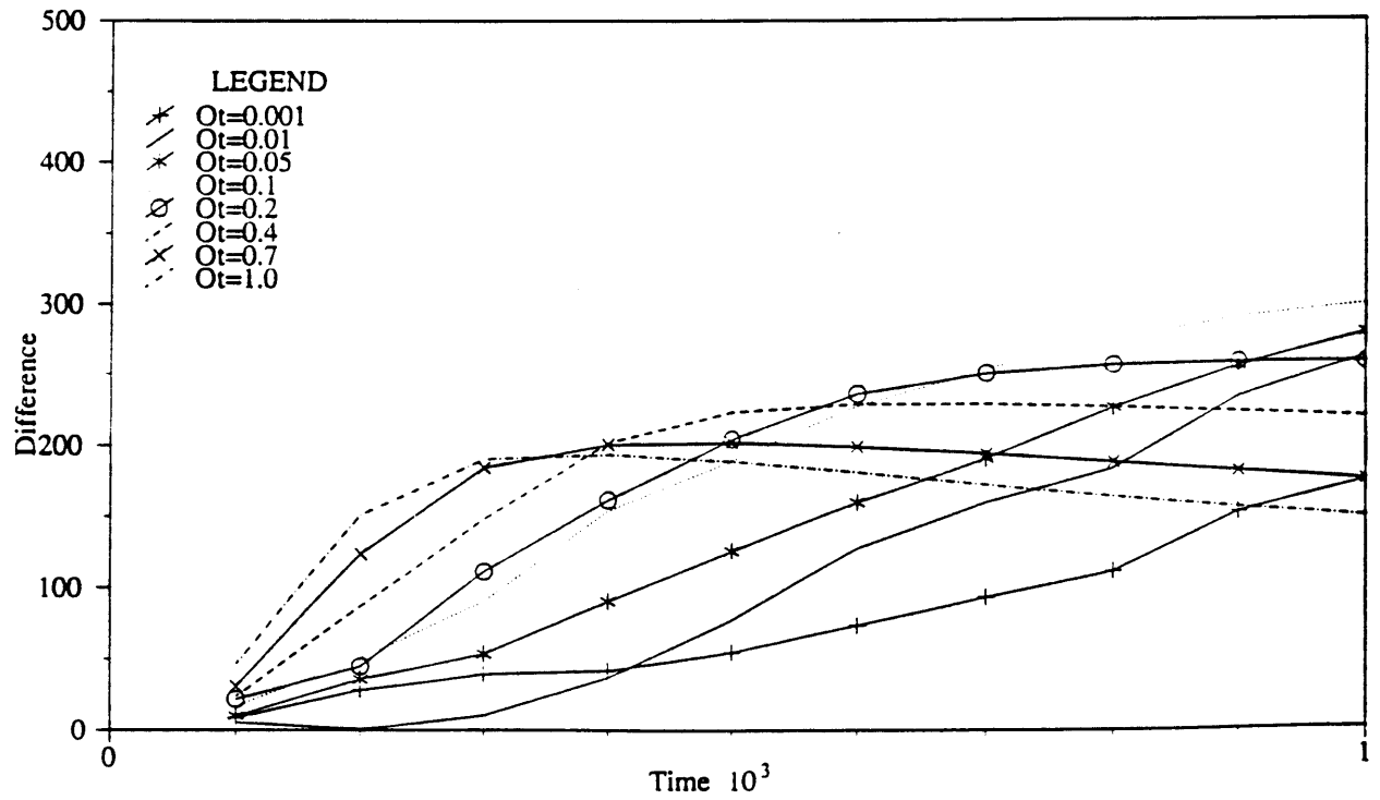
Figure 4-26: Relief Difference Under O_t Variations. Arithmetic Scale
