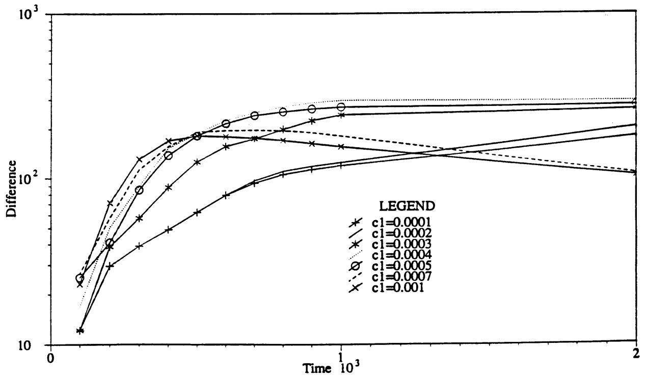
Figure 4-16: Relief Difference Under c 1 Variations During Network Growth
