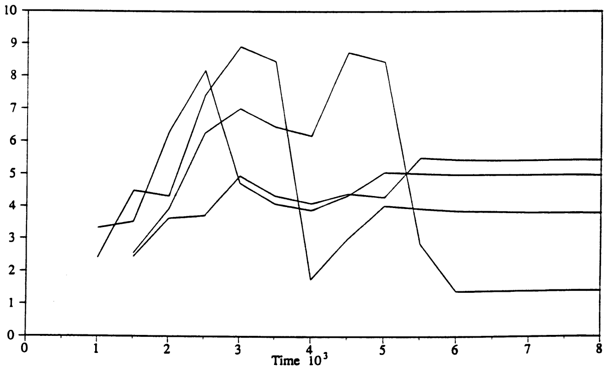
Figure 3-31: Strahler Area Ratio. Order 2-3
