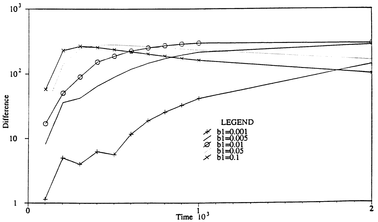
Figure 4-34: Relief Difference Under \beta_1 Variations During Network Growth
