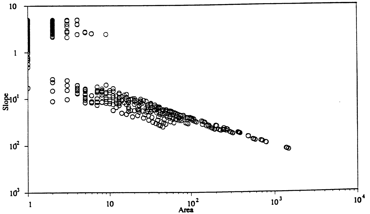
Figure 3-49: Area-Slope Renormalization. All Nodes Included. Case 32. Time 10000
