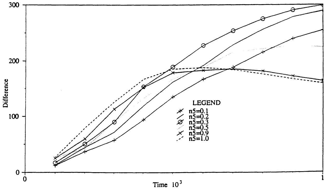
Figure 4-32: Relief Difference Under n 5 Variations. Arithmetic Scale
