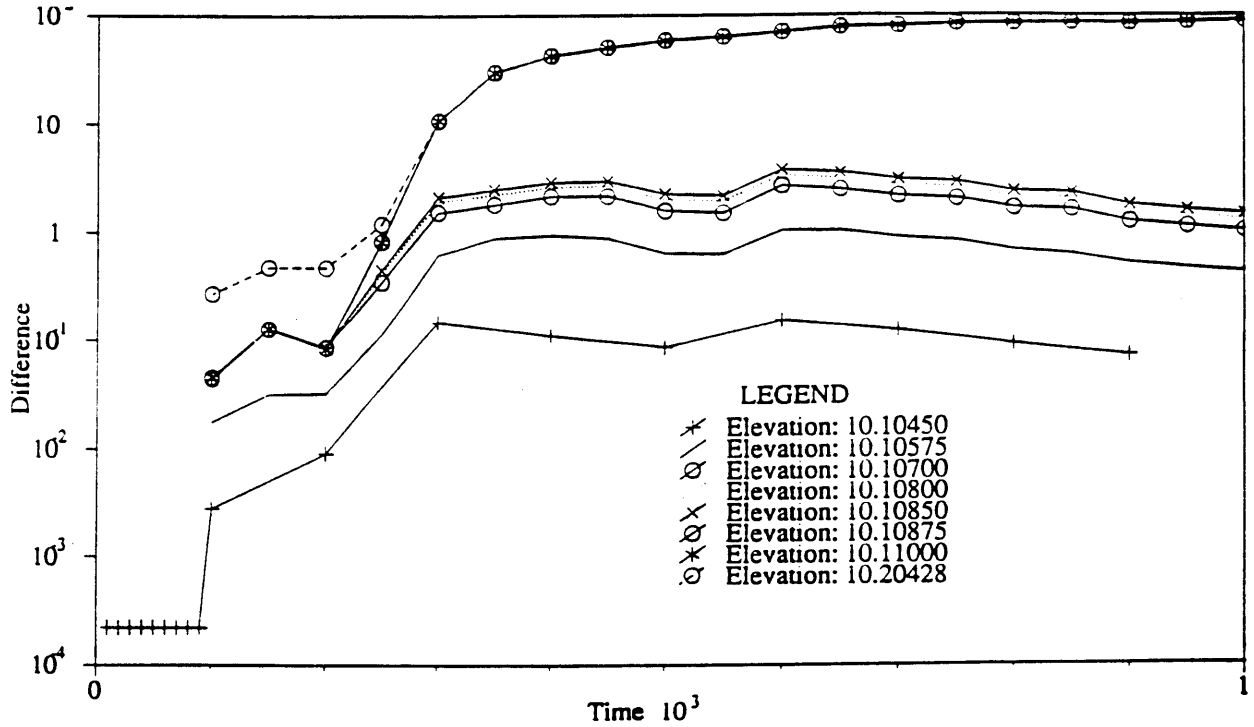
Figure 4-9: Perturbation Threshold One-Node Perturbations. Upward Perturbations Original Node Elevation 10.10428
