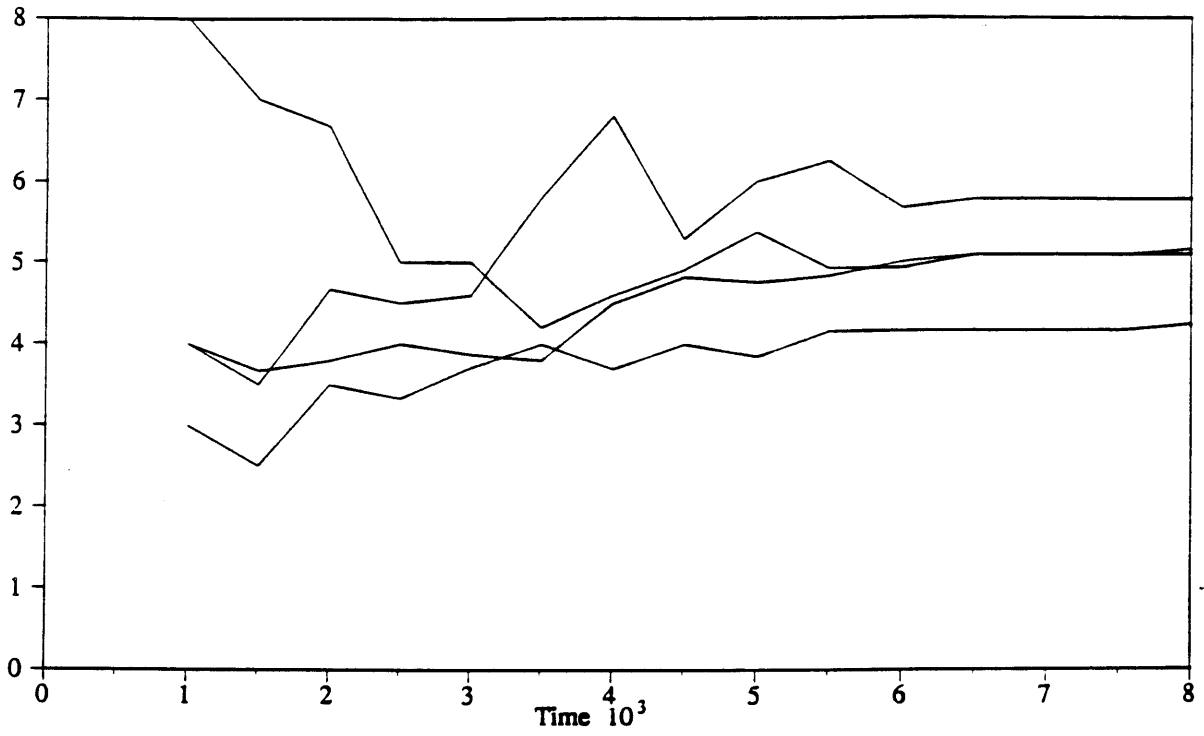
Figure 3-24: Strahler Bifurcation Ratio. Order 1-2
