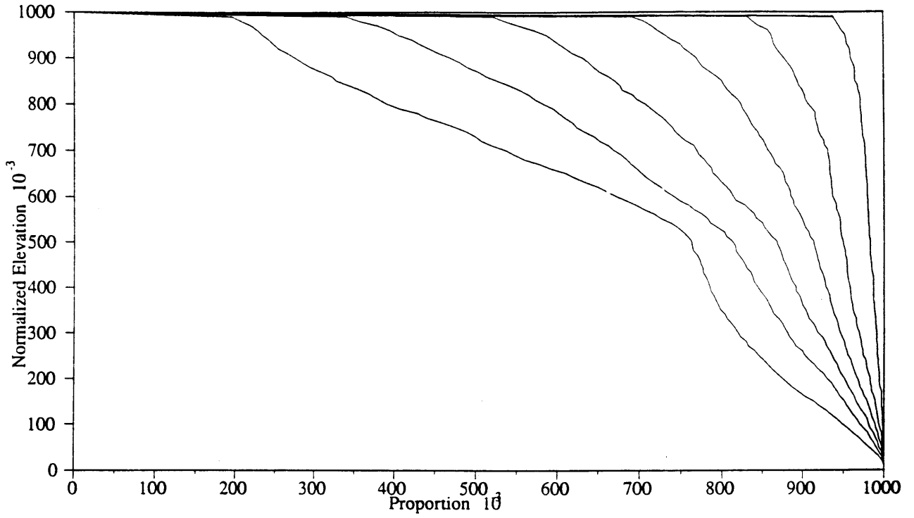
Figure 3-67: Hypsometric Curve Evolution TSC=0.920 \times 10^3
