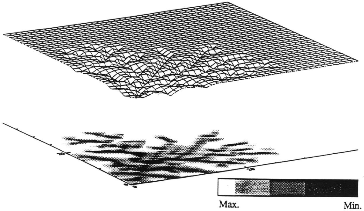
Figure 3-54: Elevations at Time 3000. Case BR661SATU10
