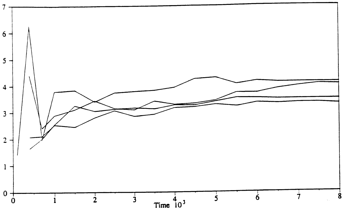
Figure 3-34: Time Evolution of Mean Link Length
