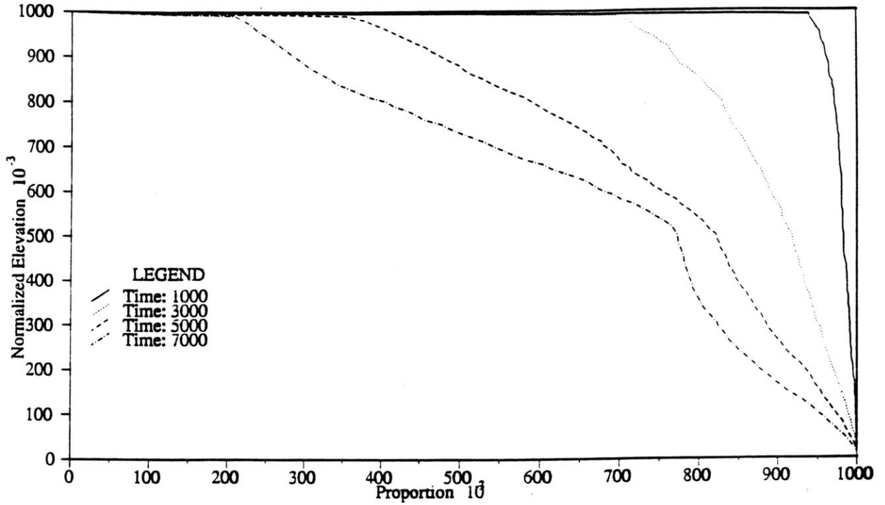
Figure 3-22: Hypsometric Curve Variation in Time
