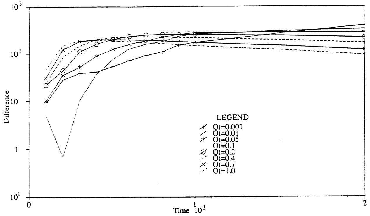
Figure 4-25: Relief Difference Under O_t Variations During Network Growth
