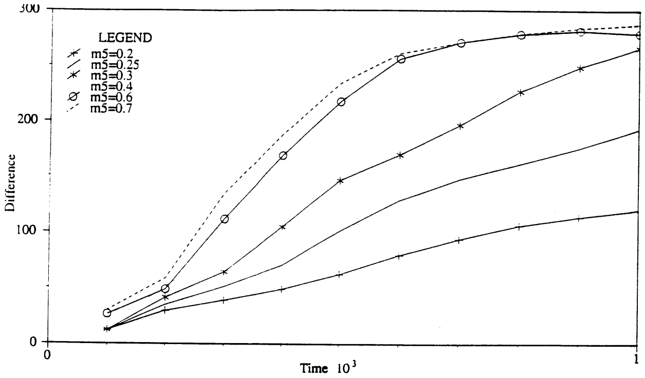
Figure 4-29: Relief Difference Under m 5 Variations. Arithmetic Scale
