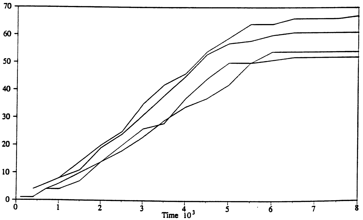
Figure 3-33: Time Evolution of Magnitude
