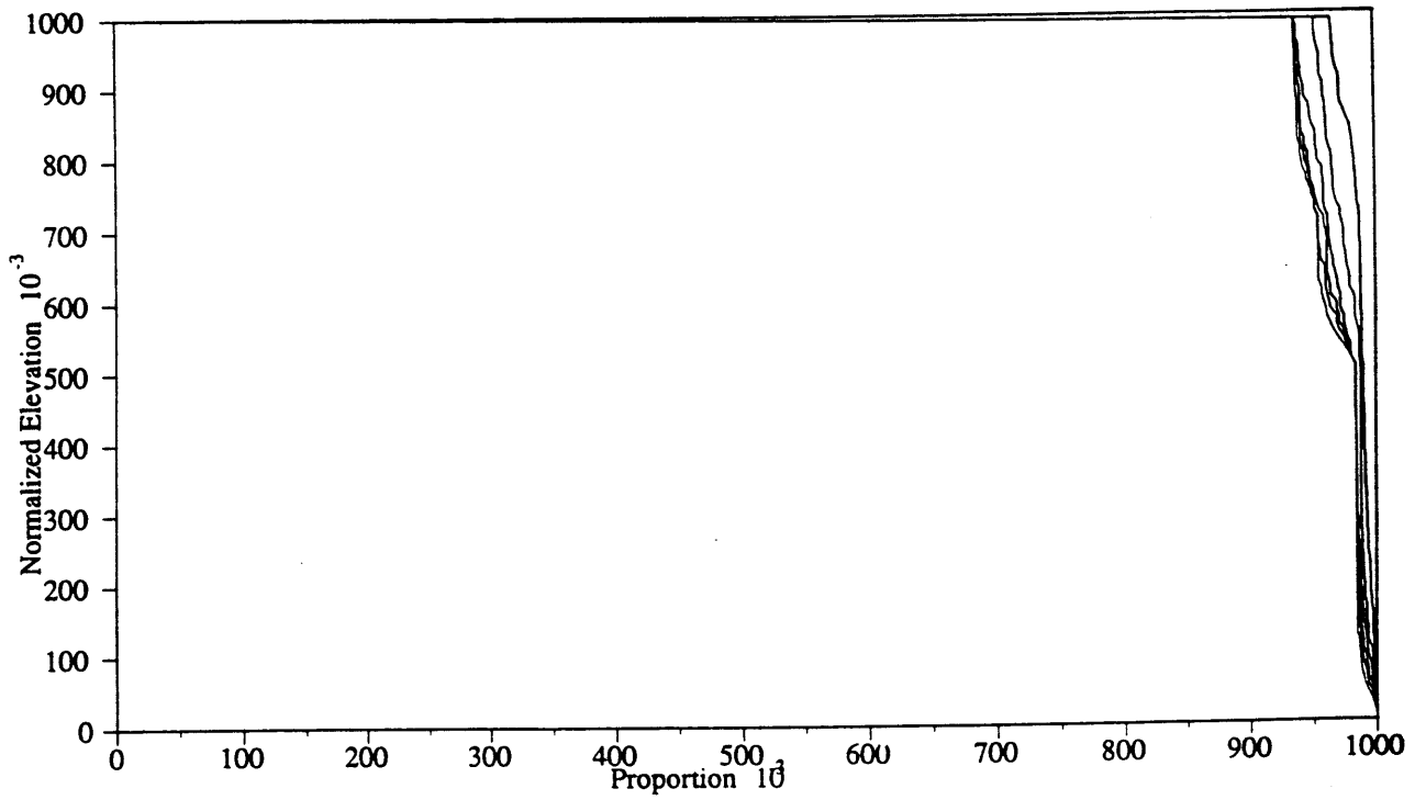
Figure 3-68: Hypsometric Curve Evolution TSC=4.60 \times 10^3
