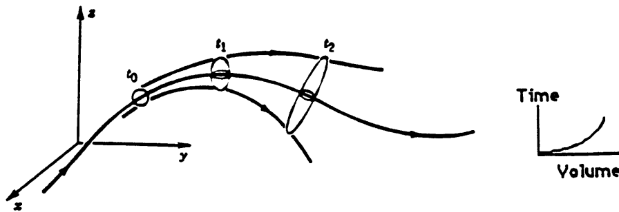
Figure 4-3: The Divergence of Volumes in Chaotic Systems
