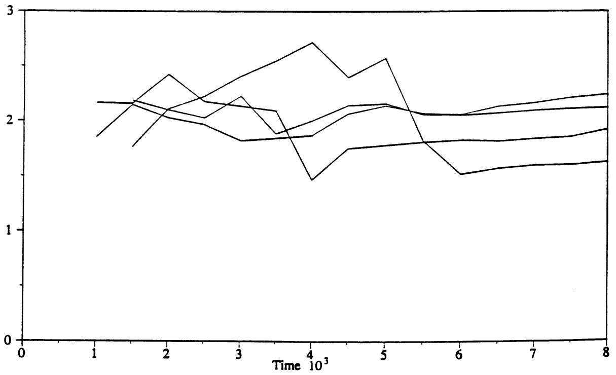
Figure 3-29: Strahler Slope Ratio. Order 2-3
