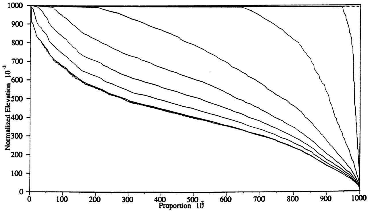
Figure 3-36: Hypsometric Curve Evolution. Episodic Uplift Case 10
