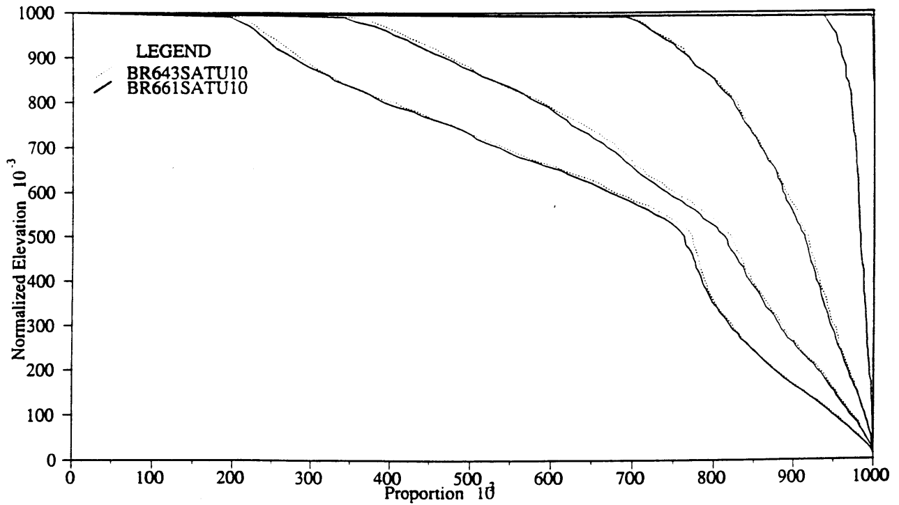
Figure 3-59: Hypsometric Curve Evolution. Cases BR643SATU10 and BR661SATU10
