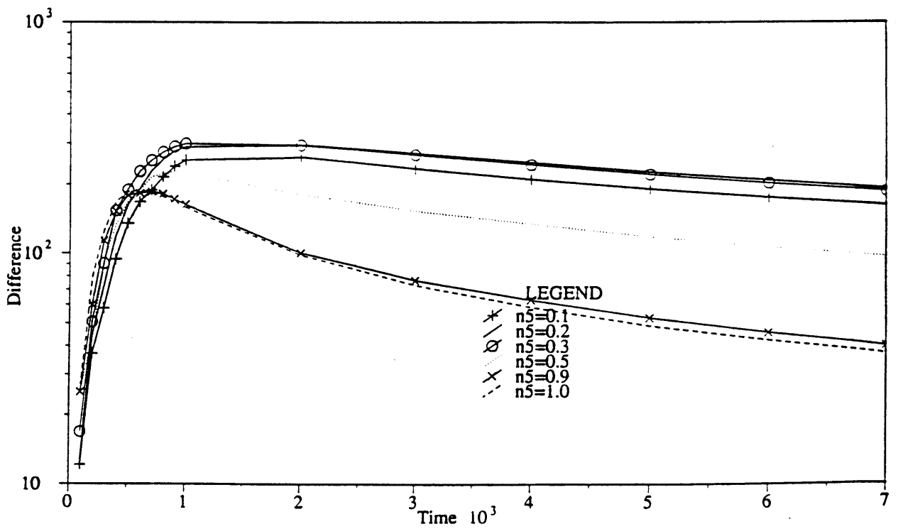
Figure 4-30: Relief Difference Under n 5 Variations
