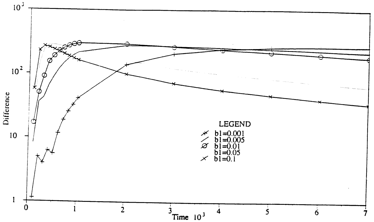
Figure 4-33: Relief Difference Under \beta_1 Variations
