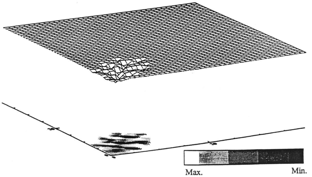
Figure 3-53: Elevations at Time 1000. Case BR661SATU10
