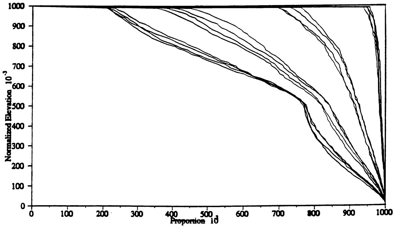
Figure 3-35: Time Evolution of Hypsometric Curve
