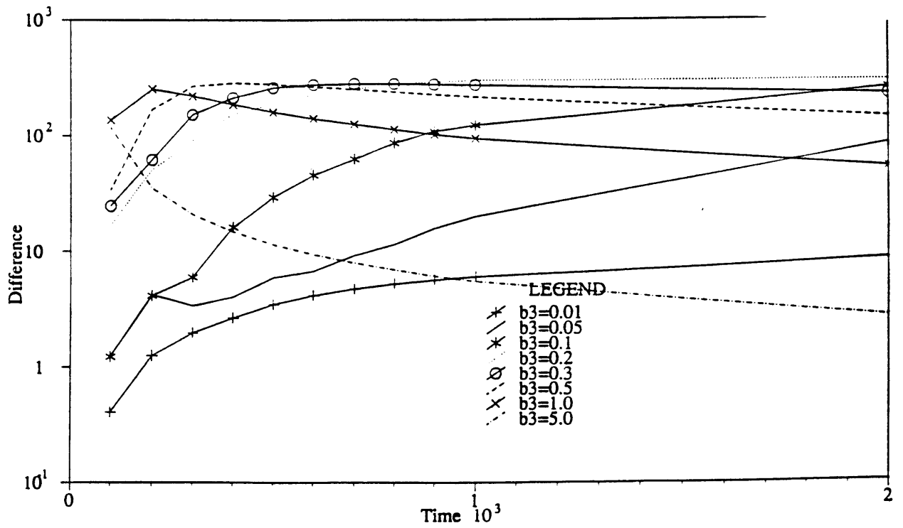
Figure 4-22: Relief Difference Under \beta_3 Variations During Network Growth
