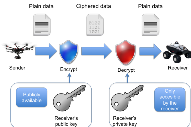
Fig. 7. Public key cryptography allows robots to be sure that the content of a message can only be read by the owner of the corresponding sending address.
