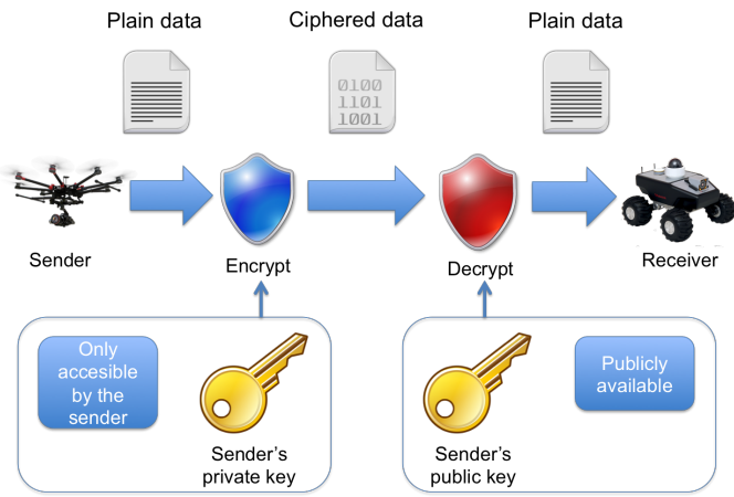
Fig. 8. Digital signature cryptography provides a way to prove the ownership of a specific address — public key.
